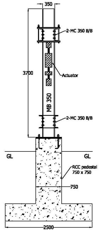
SIDE VIEW OF REACTION FRAME
