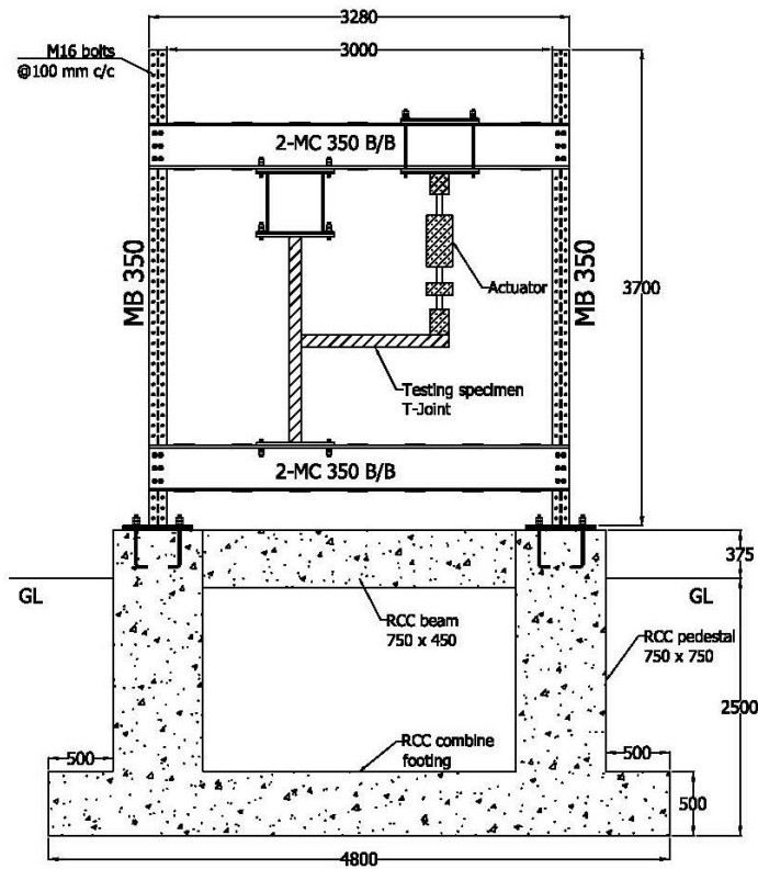
FRONT VIEW OF REACTION FRAME
